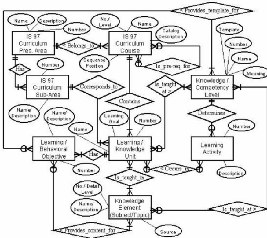
Figure 1 – A Data Model for IS'97
